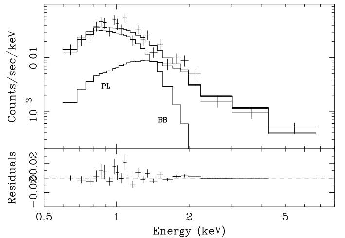
FIG. 4.— Chandra ACIS-S3 spectrum of the point source coincident with PSR B1706–44. Top panel : Data (crosses) and best-fit model (dark line) for the parameters given in Table 2; thin lines show the contribution of the power-law (PL) and blackbody (BB) components of the fit. Bottom panel : Difference between the data and model, in the same units as the top panel.
